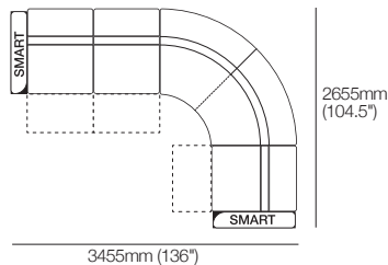
Nimbus 4-Seater Recliner with Corner Module and Smart Pockets | 4-STR 800R
