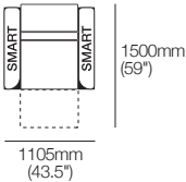
Nimbus Recliner Armchair with Compact SMART Pockets 1105mm W | Armchair 700RC SMART
