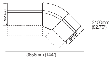
Nimbus 4-Seater Recliner with 45 Degree Curve Corner and Smart Arms 800R
