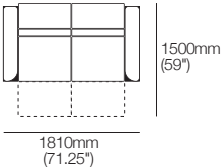
Nimbus 2-Seater Recliner with Compact Arms 1810mm W | 2-STR 700RC
