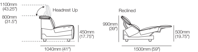
Modules 700F | 800F | 900F (Chair & Chaise) Side View
