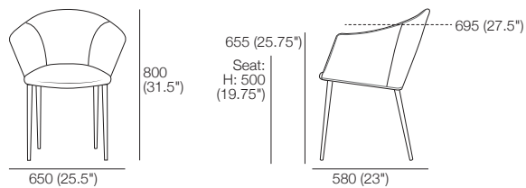
Dining Chair (Upholstered) Leather Detail Indicated Front View | Side View
