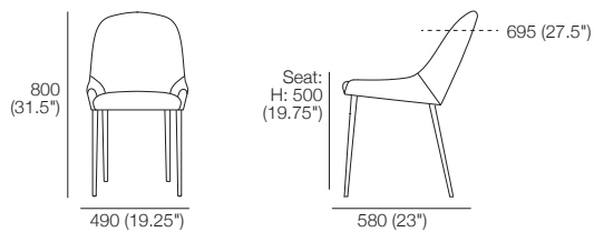
Armless Dining Chair (Upholstered) Leather Detail Indicated Front View | Side View
